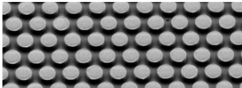
PDMS surface with a hexagonal array of cylindrical pillars obtain through e-beam lithography. Pillar diameter 4\mu\text{m} , height 3\mu\text{m} .
