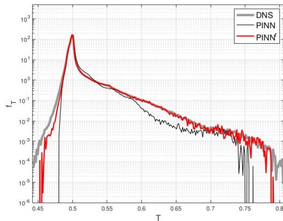
PINN predictive capabilities for Rayleigh-Bénard flow at Ra=2.10^9 [LAS22]. Left: Example of instantaneous heat dissipation field in a 2D slice from 3D DNS. The domain over which the PINN model is trained, is depicted as a transparent box. Right: probability density function of the temperature fluctuations within the training domain. The reference PDF is computed from the full DNS while the two PINNs PDF are evaluated on the predicted test sample.
